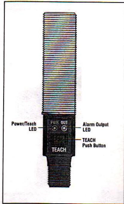
Figure 1. Sensor features
