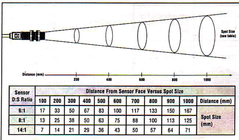
Figure 2. Detection spot size versus distance from sensor
